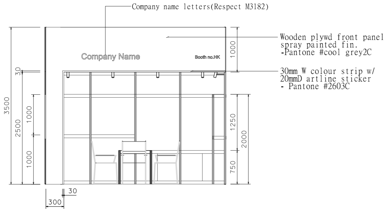
FRONT ELEVATION
